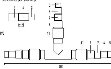
Discharge piping
