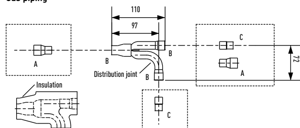
Gas piping
