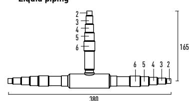
Liquid piping
