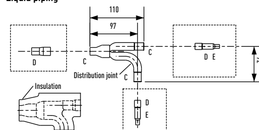
Liquid piping
