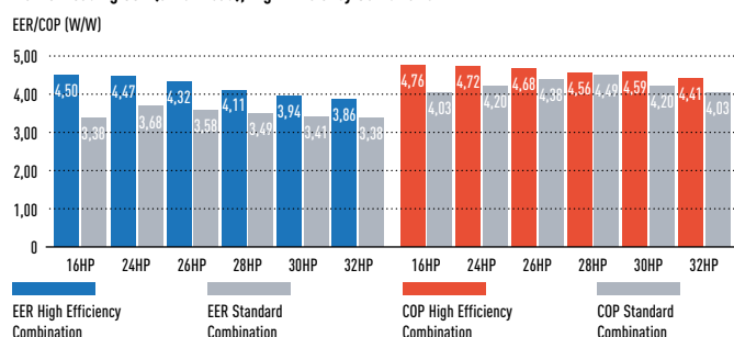
Market-leading COP (at full load), High Efficiency Combination.
