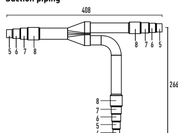
Suction piping
