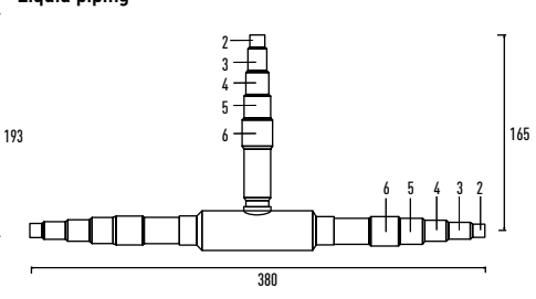
Liquid piping
