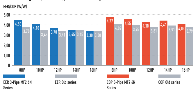
Market-leading COP (at full load), standard efficiency.
